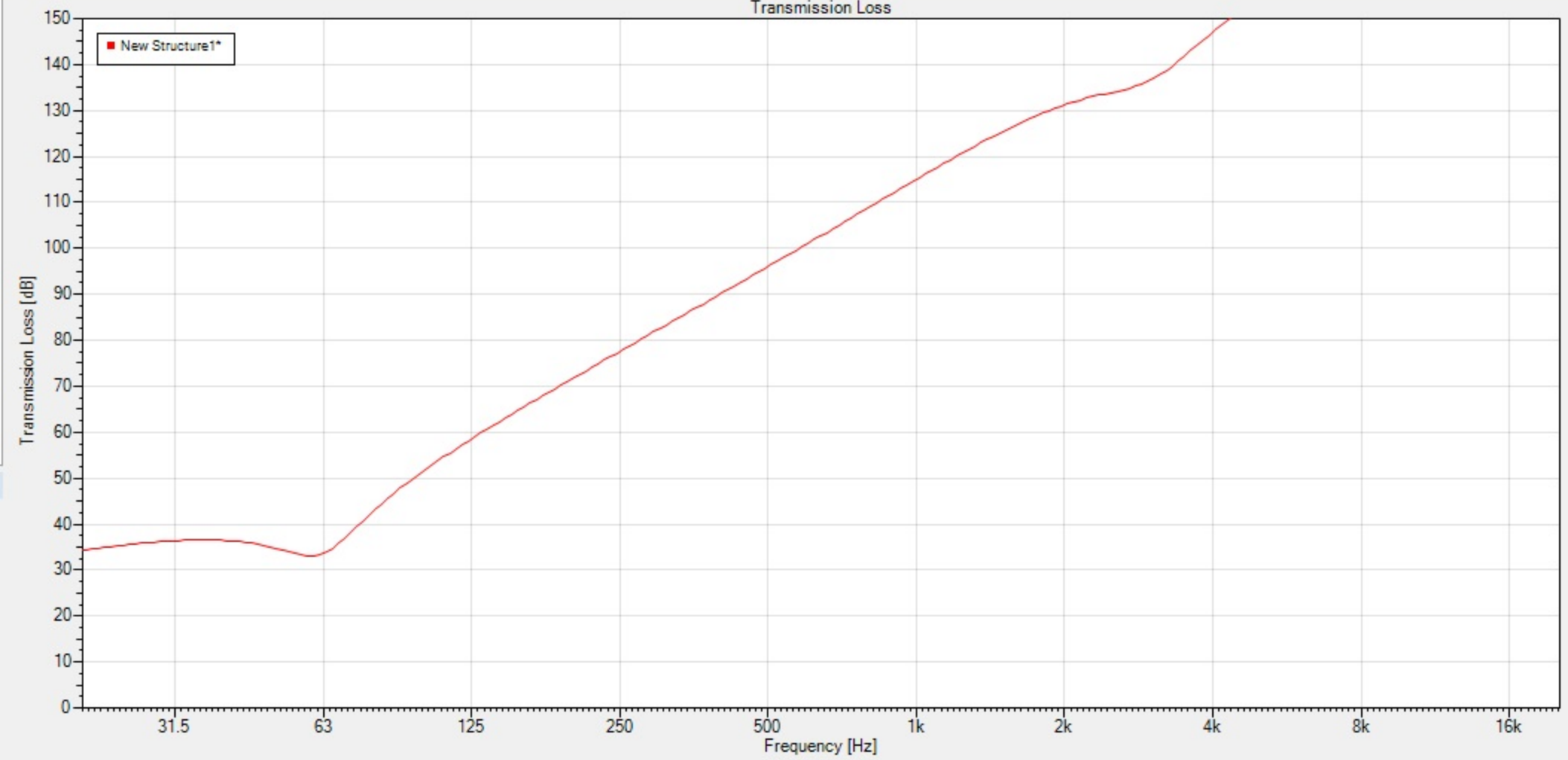
Transmission Loss
